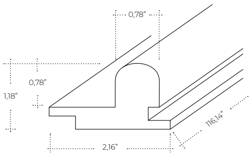
Round Profile
