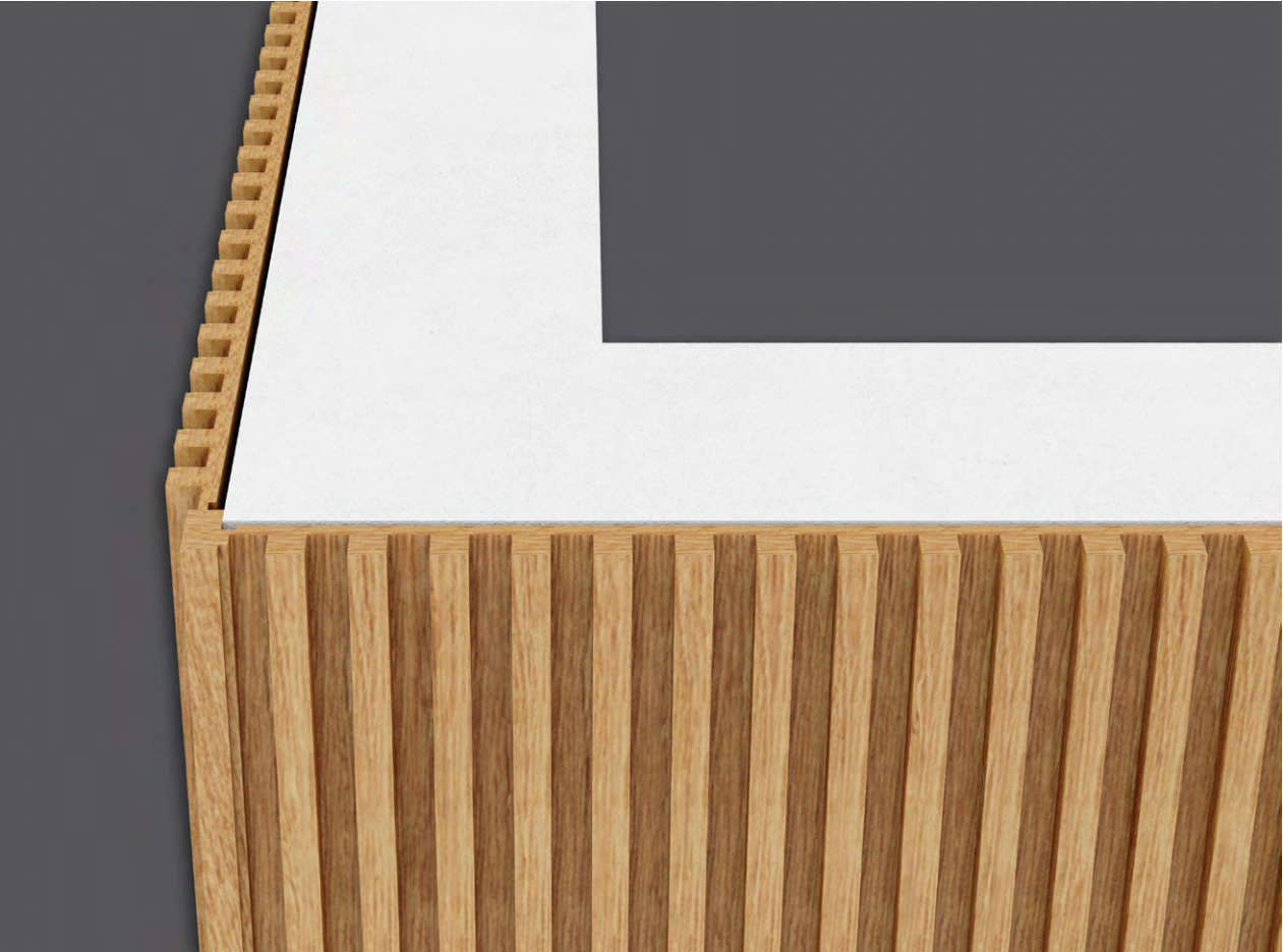
External Corner Assembly
