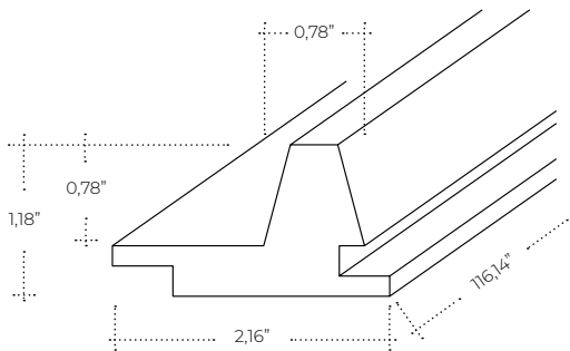
Triangular Profile
