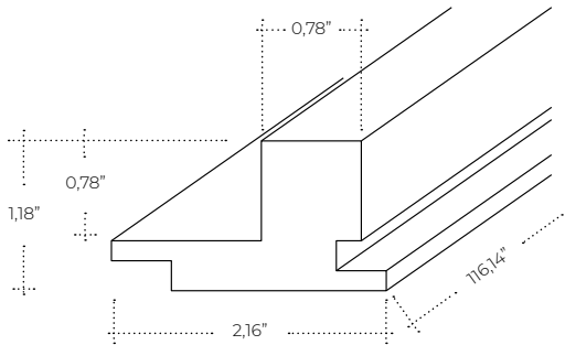
Square Profile
